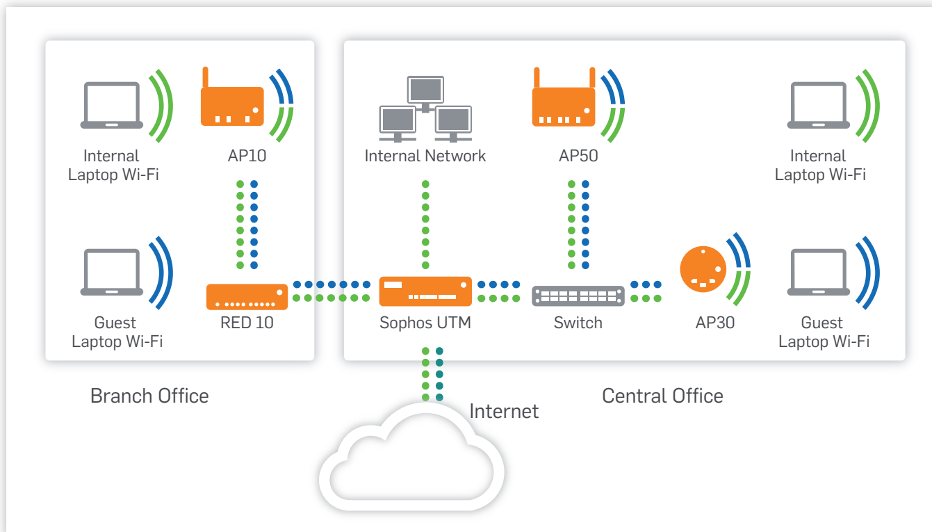
Deployment scenario of Sophos UTM Wireless Protection
